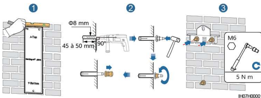
Figure 4-8 Installation des boulons expansibles
