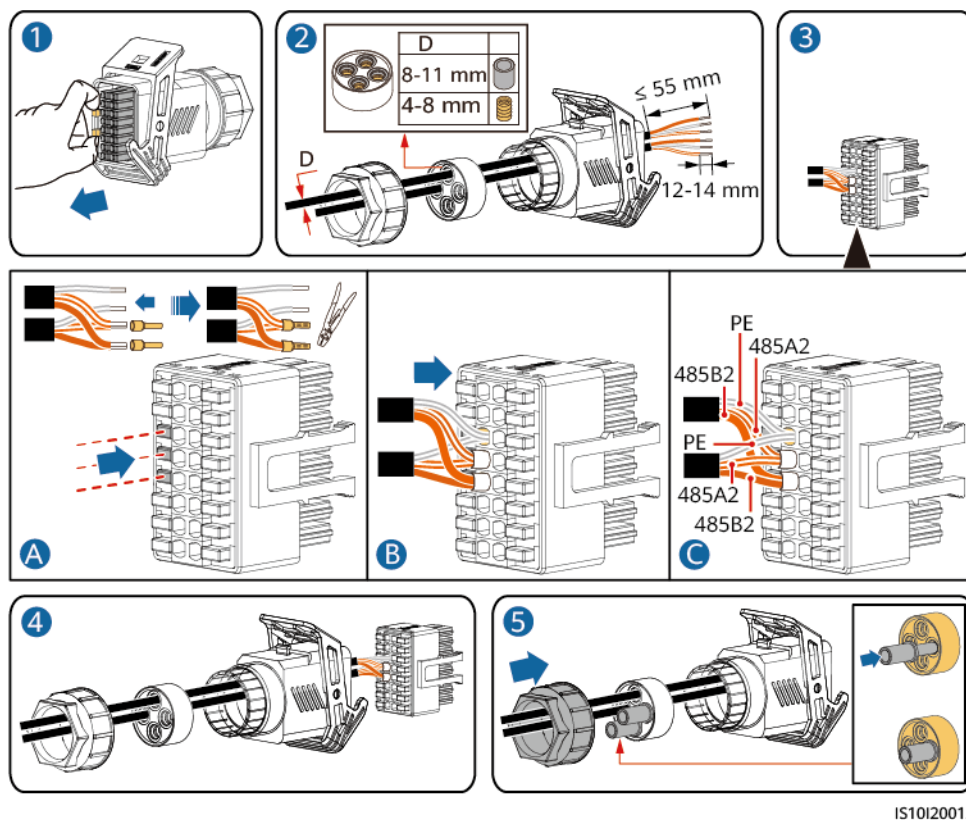
Figure 5-27 Installation du câble
